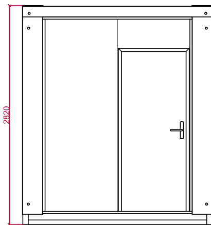
ALZADO PRINCIPAL
