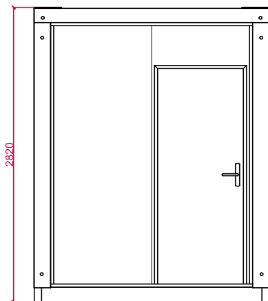
ALZADO PRINCIPAL
